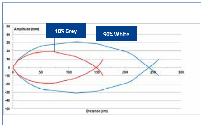
Diffused proximity
